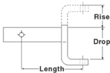
To Measure Ball Mount Rise:
