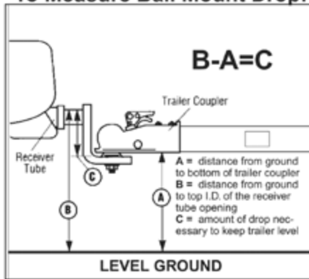
To Measure Ball Mount Drop:
