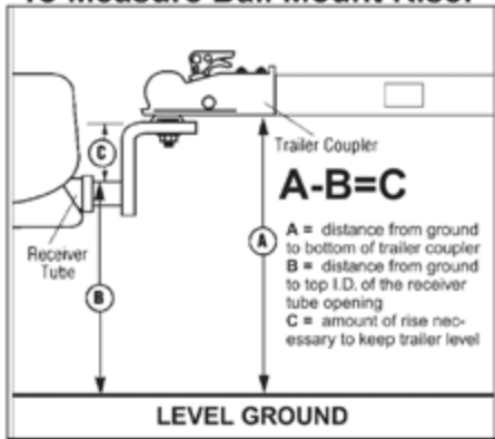
To Measure Ball Mount Rise:
